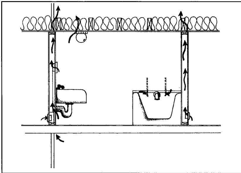
Figure 1 Attic bypasses from the bathroom.
