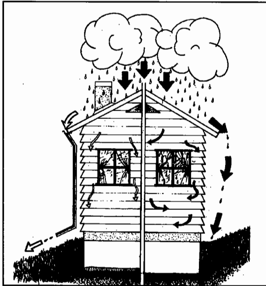
Figure 7 Gutters, a slope away from the house and drainage tile in the foundation keep the left side of this house dry. No gutters, a slope toward the house, and no drainage tile expose the right side to moisture damage.
