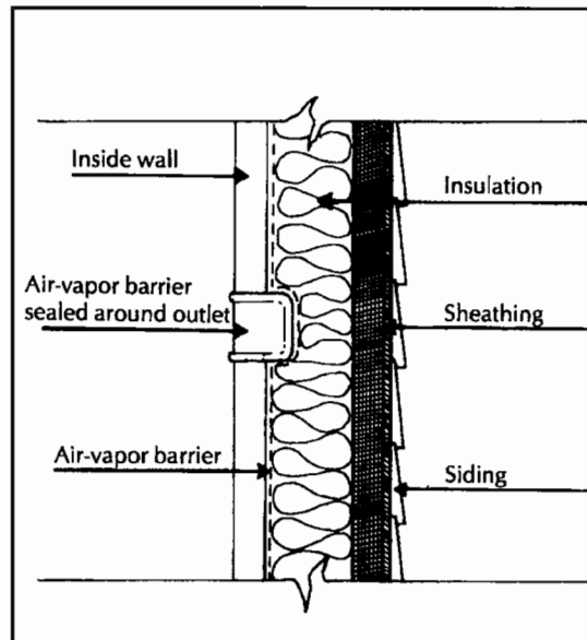
Figure 3 Air-vapor barrier placement
