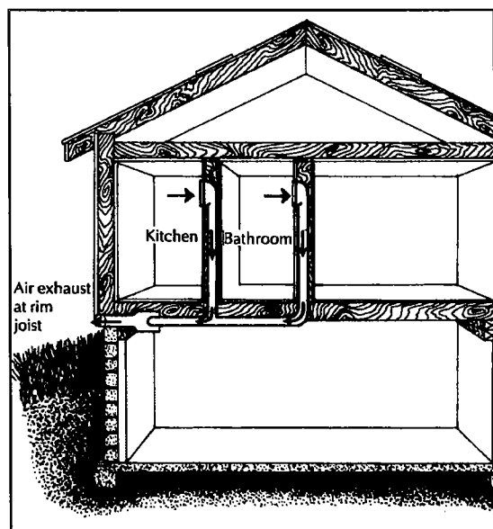
Figure 4 Mechanical ventilation
