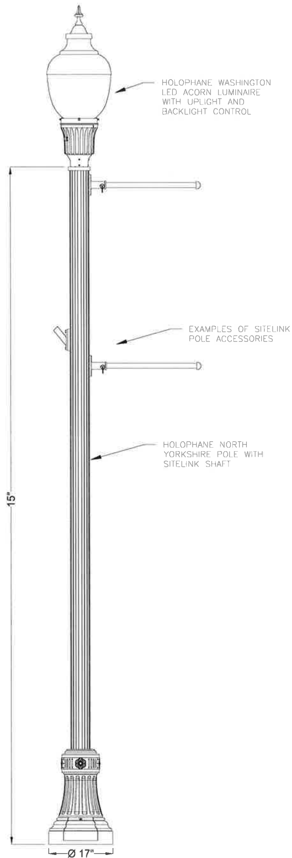
HISTORIC POLE AND LUMINAIRE OPTION
