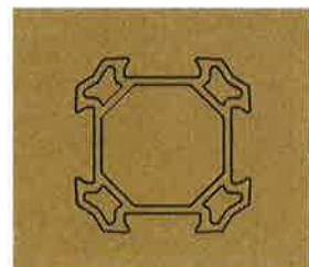
Medium Duty (T2) Four track pole 5.75" square
