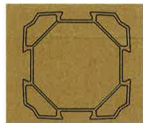
Heavy Duty (T3) Four track pole 8.5" square
